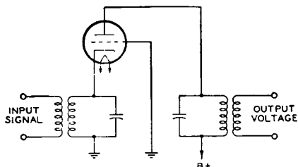
Fig. 47—Cathode-drive circuit.
