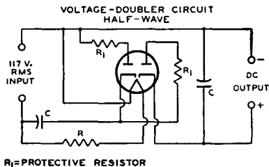
Fig. 20—Full-wave and half-wave voltage-doubler circuits showing heater-supply connections.
