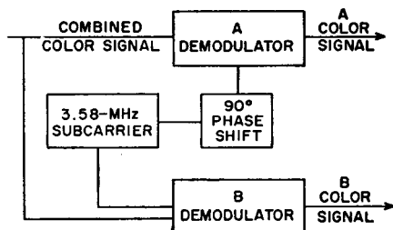
Fig. 95—Separation of combined color signal into two signals at the receiver.
