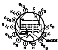
ANODE - G_2 + G_4 + C_L FOCUSING ELECTRODE - G_3
