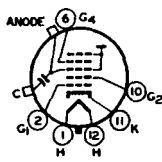
12L ANODE = G_3 + G_5 + C_1 FOCUSING ELECTRODE = G_4
