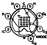
9EP ANODE = G_3 + G_5 + C_1 FOCUSING ELECTRODE = G_4
