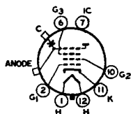
12C ANODE = G_4 + C_1 FOCUSING ELECTRODE = G_3
