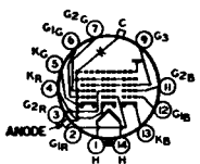
ANODE - G_4 + G_5 + C_L FOCUSING ELECTRODE - G_3
