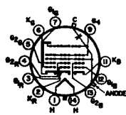
ANODE - G_3 + G_5 + C_L FOCUSING ELECTRODE - G_4
