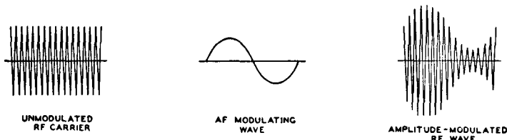
Fig. 21—Waveforms showing effect of amplitude modulation on an rf wave.
