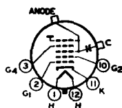
12AB ANODE = G_3 + G_5 + C_1 FOCUSING ELECTRODE = G_4
