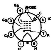
8JR ANODE = G_4 + C_1 FOCUSING ELECTRODE = G_3
