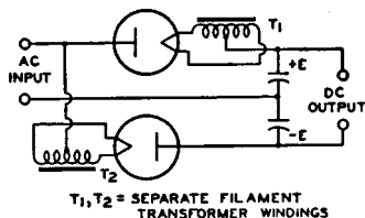
Fig. 19—Full-wave voltage-doubler circuit.
