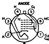
77G ANODE = G_3 + G_5 + C_1 AUTOMATIC FOCUSING
