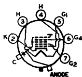
77A ANODE = G_3 + G_5 + C_1 FOCUSING ELECTRODE = G_4
